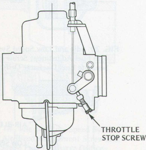
FIG. 23 Carburetor with Disc Type Throttle Valve
