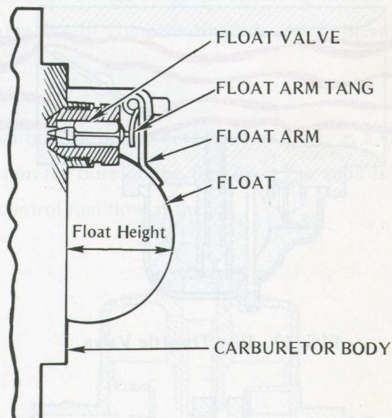
FIG. 9 Float Height
