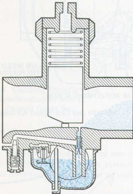
FIG. 18 Idle and Low Speed System with Air-Bleed Adjustment Screw and Single Fuel Discharge Orifice
