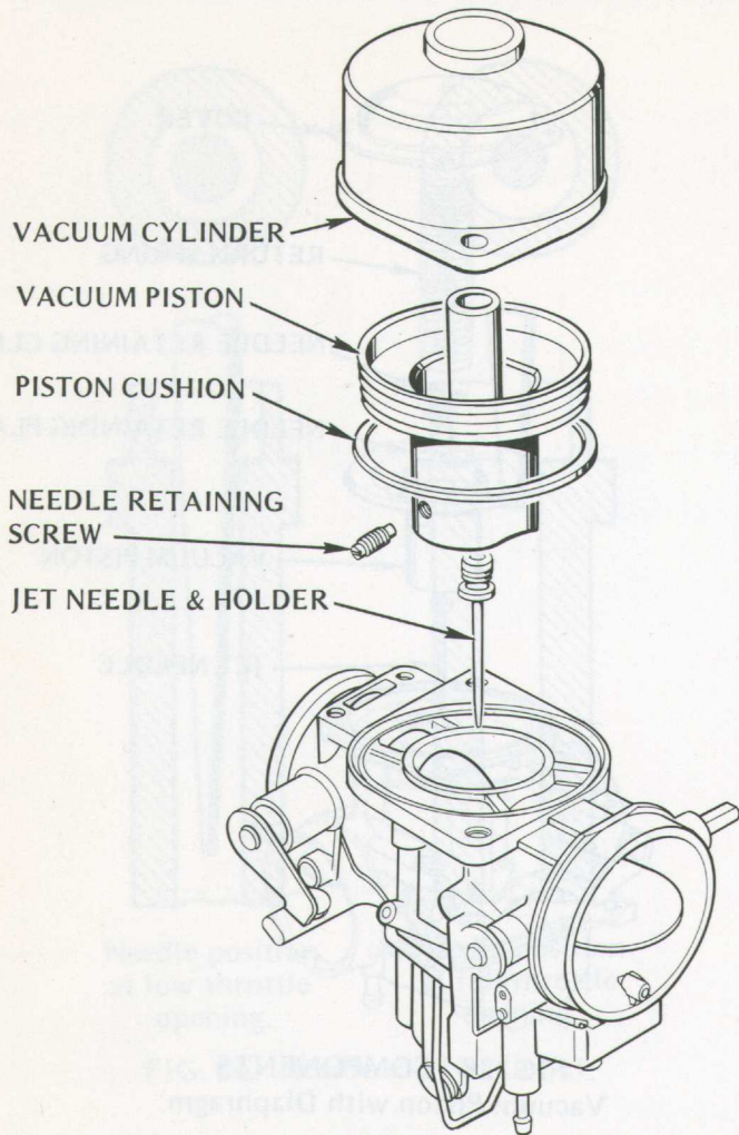
FIG. 30 COMPONENTS Vacuum Piston without Diaphragm
