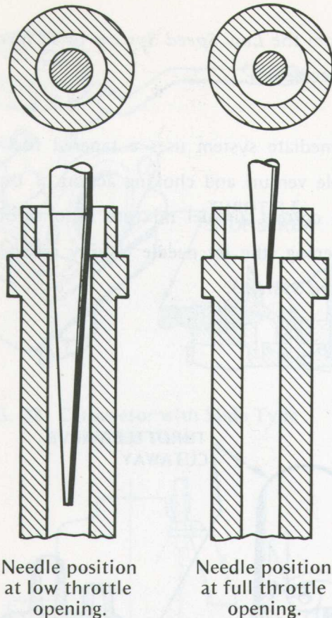
FIG. 26 Needle and Needle Jet
