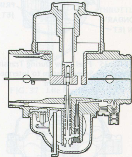
FIG. 33 Low rpm and Full Throttle Opening
