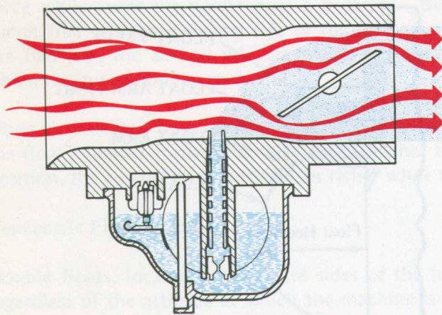
FIG. 11 Disc Throttle Valve
