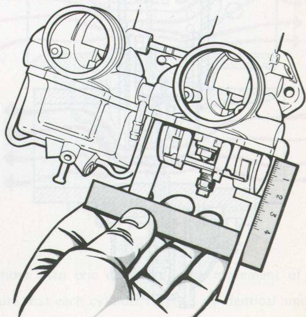
FIG. 10 Float Height Gauge
