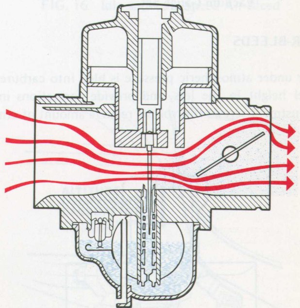
FIG. 13 Disc Throttle Valve and Vacuum Piston
